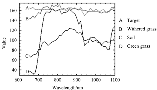
Fig. 6 Spectral curves of the main objects in the hyperspectral remote sensing image target detection experiment
