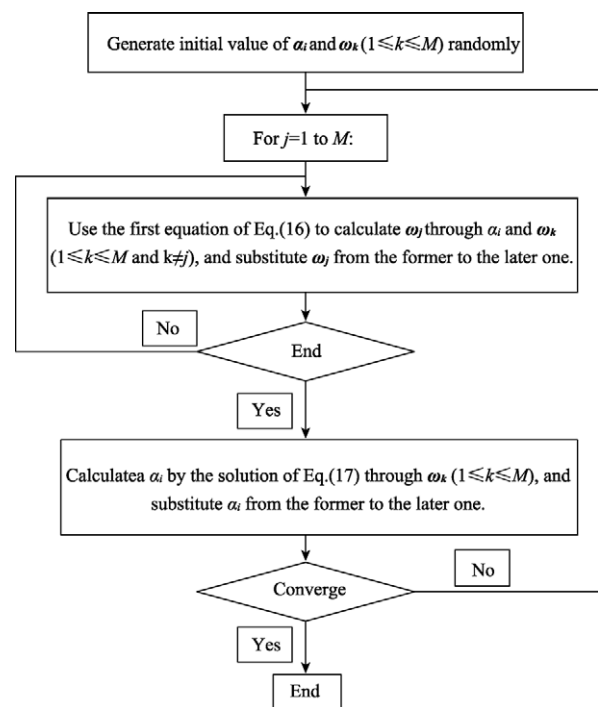
Fig. 4 Alternating projection procedure
