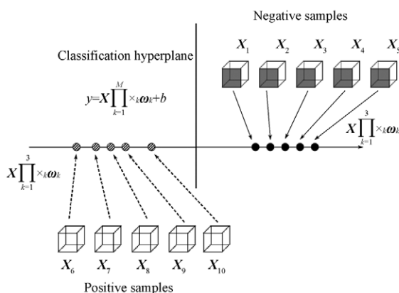
Fig. 3 Tensor hyperplane for 3-order tensor classification
